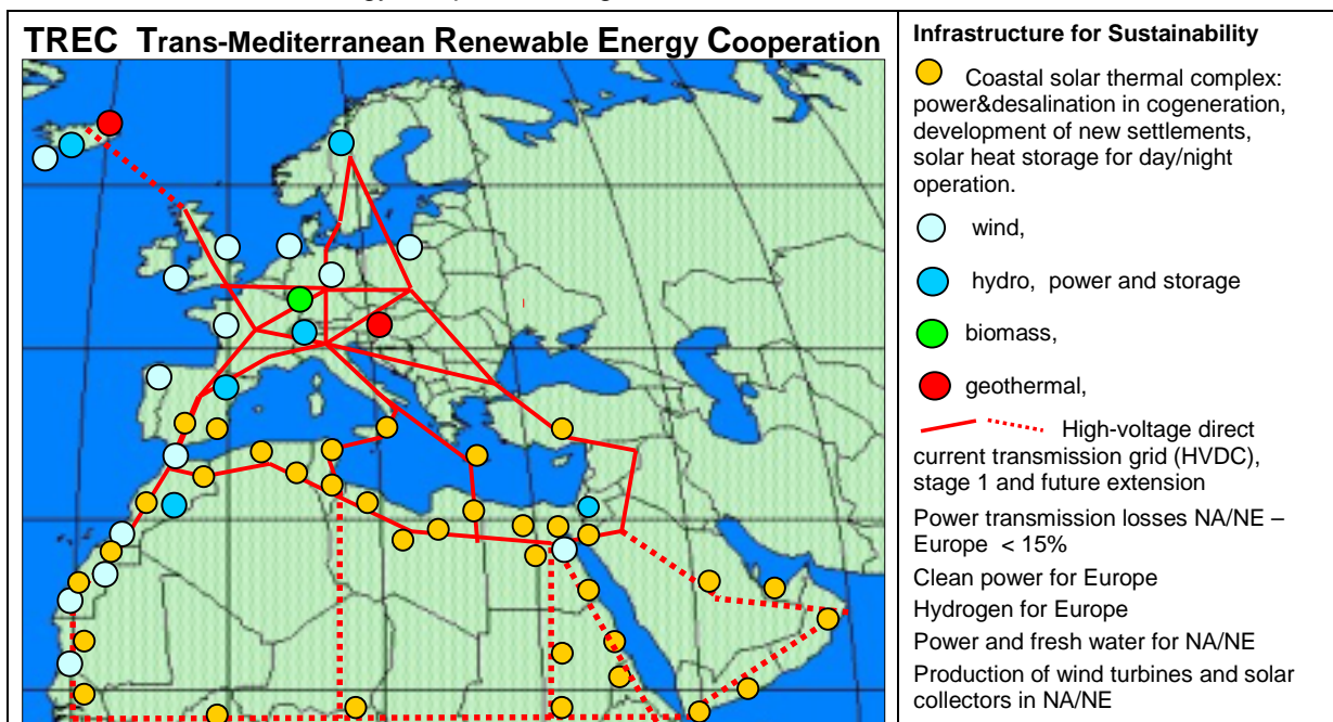
Figure 1: Renewable energy optimisation by long-distance power interconnections and synergy exploitation of resources in Europe and North Africa/Near East (hereafter: NA/NE).
