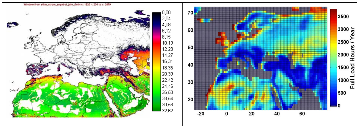
Figure 2 left: Annual average electricity generating potential of concentrating solar thermal power plants in MW/km 2 , averaged over an area of 5x5 km 2 . For annual production per km 2 (GWh/km 2 /y) multiply colour code numbers with 8760 h. White areas are excluded due to other land use and land cover. Right: Yield of a variable speed wind turbine at 80m height in terms of full load hours per year for a spatial resolution of 1.125°x1.125°, corresponding to 125kmx110km(Sahara, 70km North Sea), averaged over 10 years. For annual production multiply with rated power of the turbine. Source: DLR, ISET; radiation derived from ECMWF, NCEP/NCAR, wind from ECMWF.
